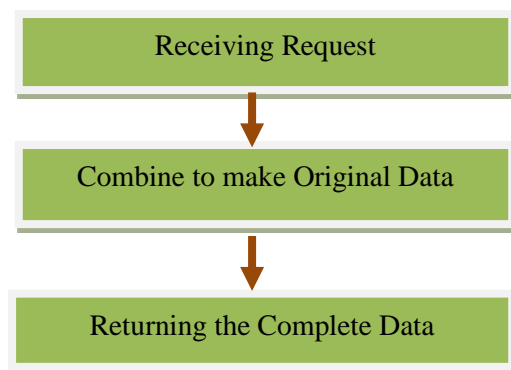
Fig.1 Data Accessing
