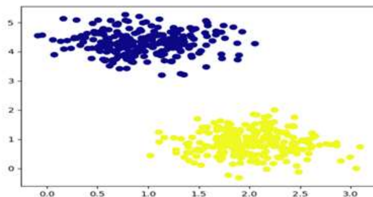
Fig.2 Scatter Plot
