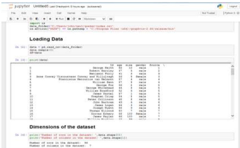
Fig.3 Loading Data
